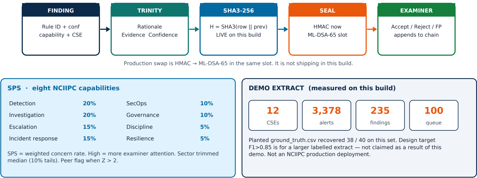
FIGURE 4 · Finding → Trinity → SHA3-256 chain → examiner seal
